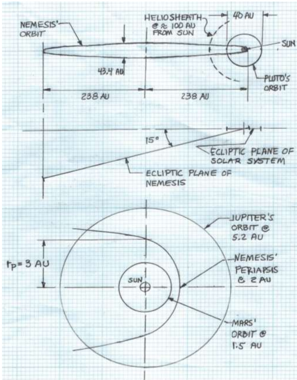
Version #2: Scale Diagram of Nemesis's Orbital Path with a Periapsis of 2 AU
