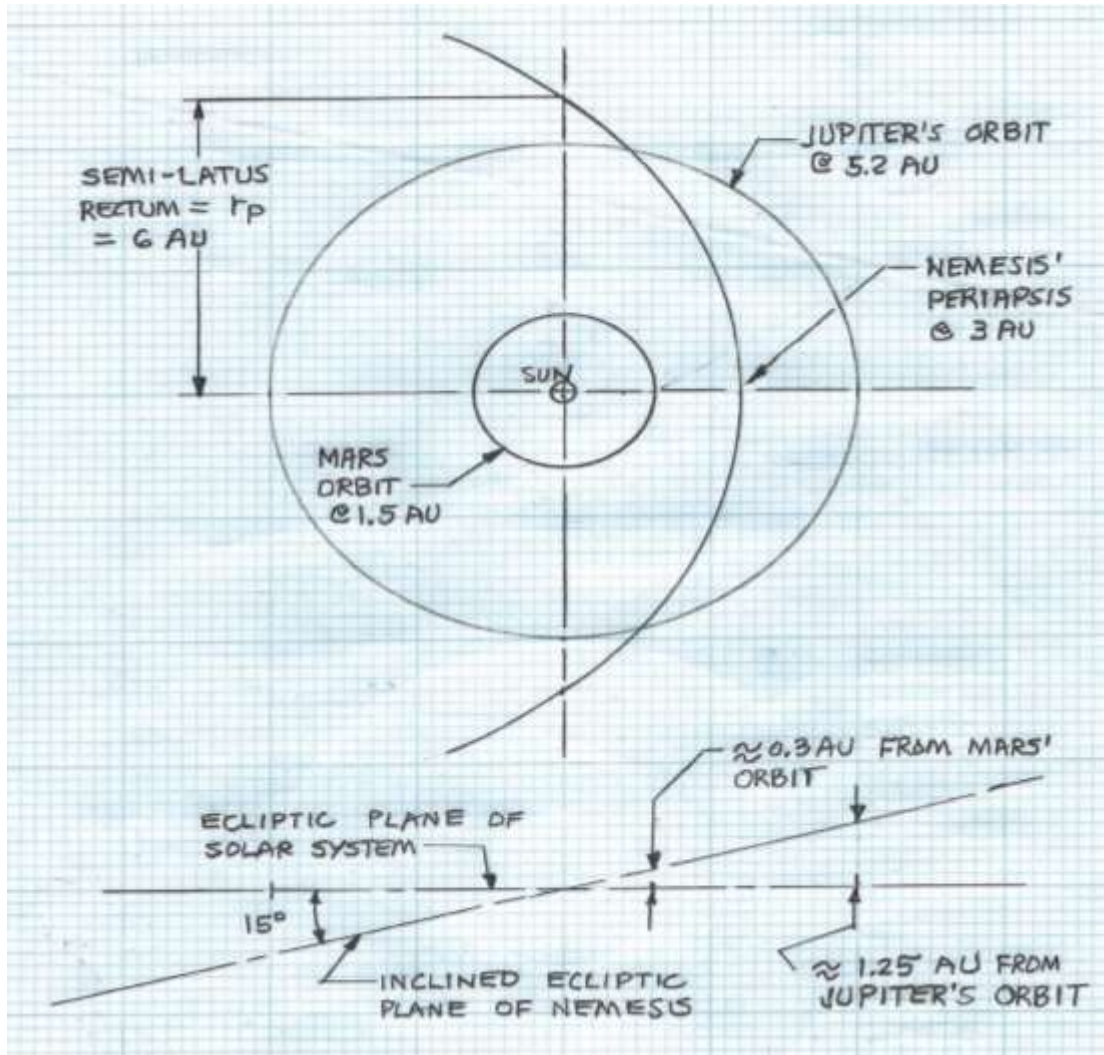
Version #1: Scale Diagram of Nemesis's Orbital Path with a Periastron of 3 AU
